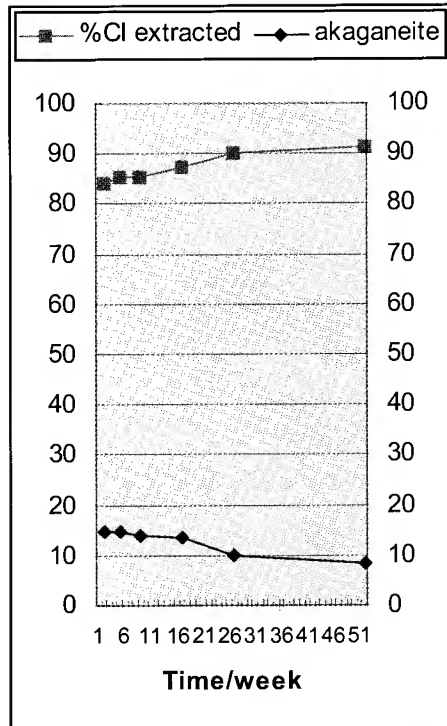
Figure 5. Removal of Chloride from \beta -FeOOH/ \text{Fe}_3\text{O}_4 mixture and transformation of \beta -FeOOH to \text{Fe}_3\text{O}_4 a function of time, in deionised water wash in closed container.
