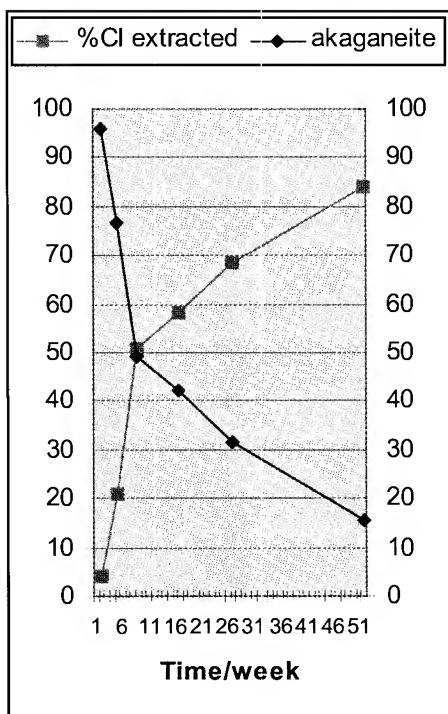
Figure 4. Removal of Chloride from \beta -FeOOH/ \text{Fe}_3\text{O}_4 mixture and transformation of \beta -FeOOH to \text{Fe}_3\text{O}_4 a function of time, in deionised water wash aerated.
