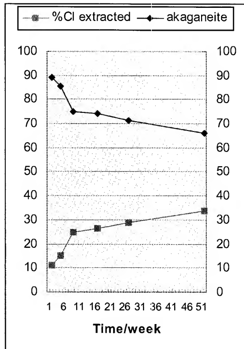
Figure 2. Removal of Chloride from \beta -FeOOH/ \text{Fe}_3\text{O}_4 mixture and transformation of \beta -FeOOH to \text{Fe}_3\text{O}_4 a function of time, in 0.5M NaOH wash aerated.
