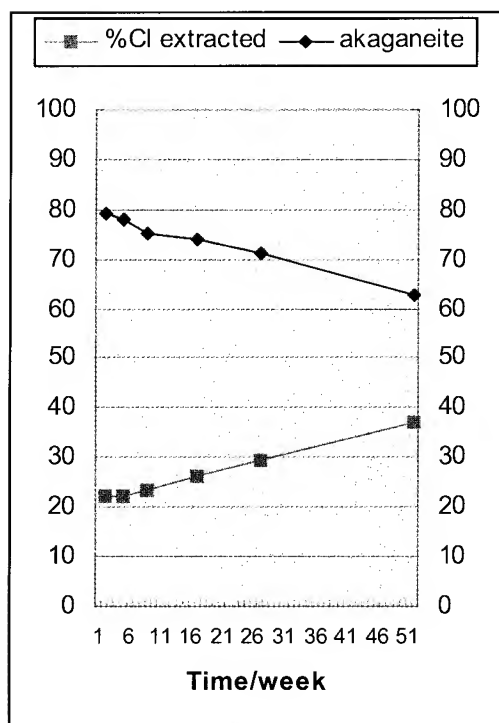
Figure 3. Removal of Chloride from \beta -FeOOH/ \text{Fe}_3\text{O}_4 mixture and transformation of \beta -FeOOH to \text{Fe}_3\text{O}_4 a function of time, in 0.5M NaOH wash in a closed container.
