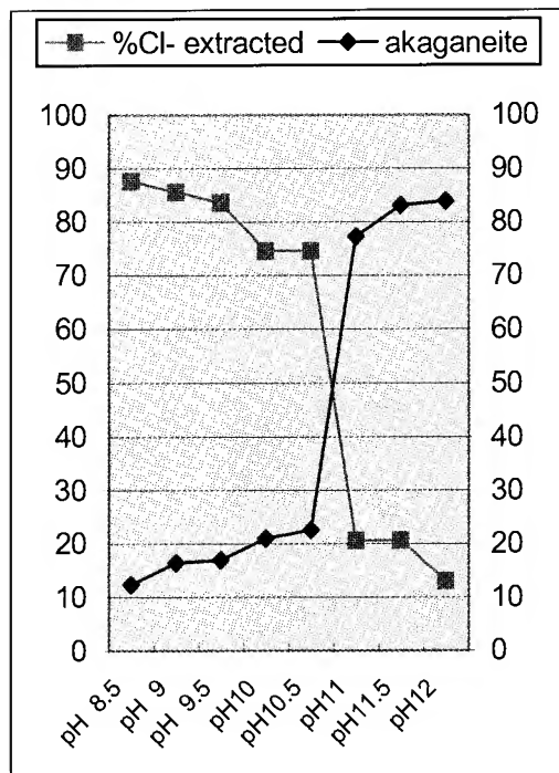
Figure 1. Percentage chloride removed from \beta -FeOOH [b] ( \beta -FeOOH/ \text{Fe}_3\text{O}_4 ) by \blacksquare washing by variable concentration of NaOH. Percentage of akaganeite remaining in the mixture as function of pH (where the original concentration of \beta -FeOOH \blacklozenge was assigned a value of 100%). Time period for washes 7 days at room temperature (approximately 20 °C).
