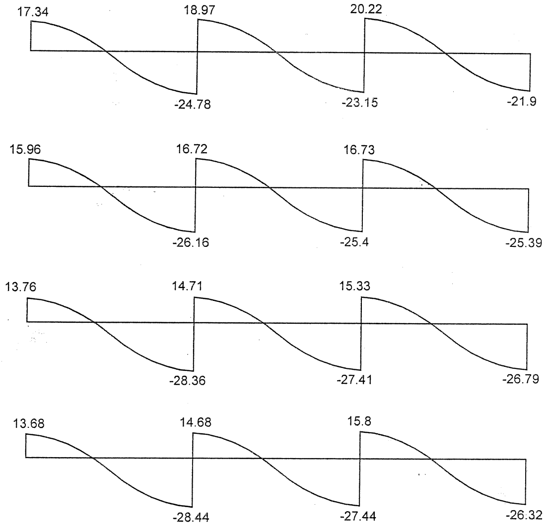
Frame F2 Shear Force U2
