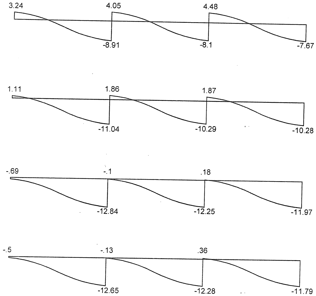
Frame F2 Shear Force U3
