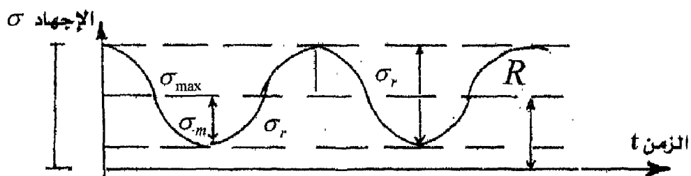
Fluctuating stress
