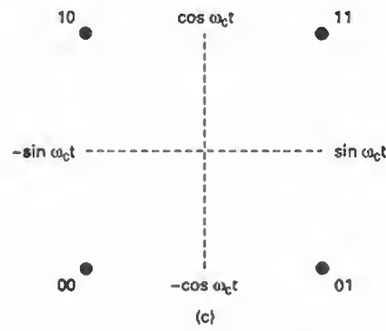
QPSK modulator: (a) truth table; (b) phasor diagram; (c) constellation diagram
