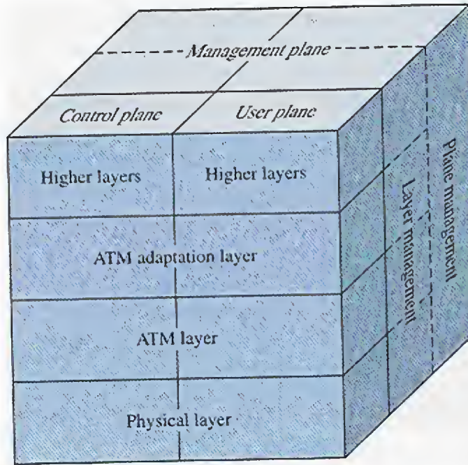
The broadband ISDN reference model
