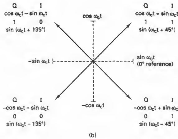
QPSK modulator: (a) truth table; (b) phasor diagram; (c) constellation diagram
